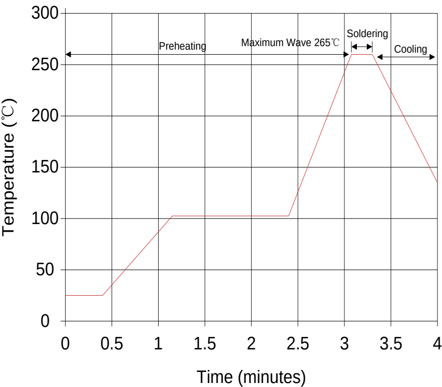
Lead-free Wave Soldering Recommendation
